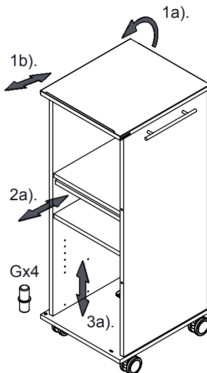
RD-4036 (estantes / shelves)
